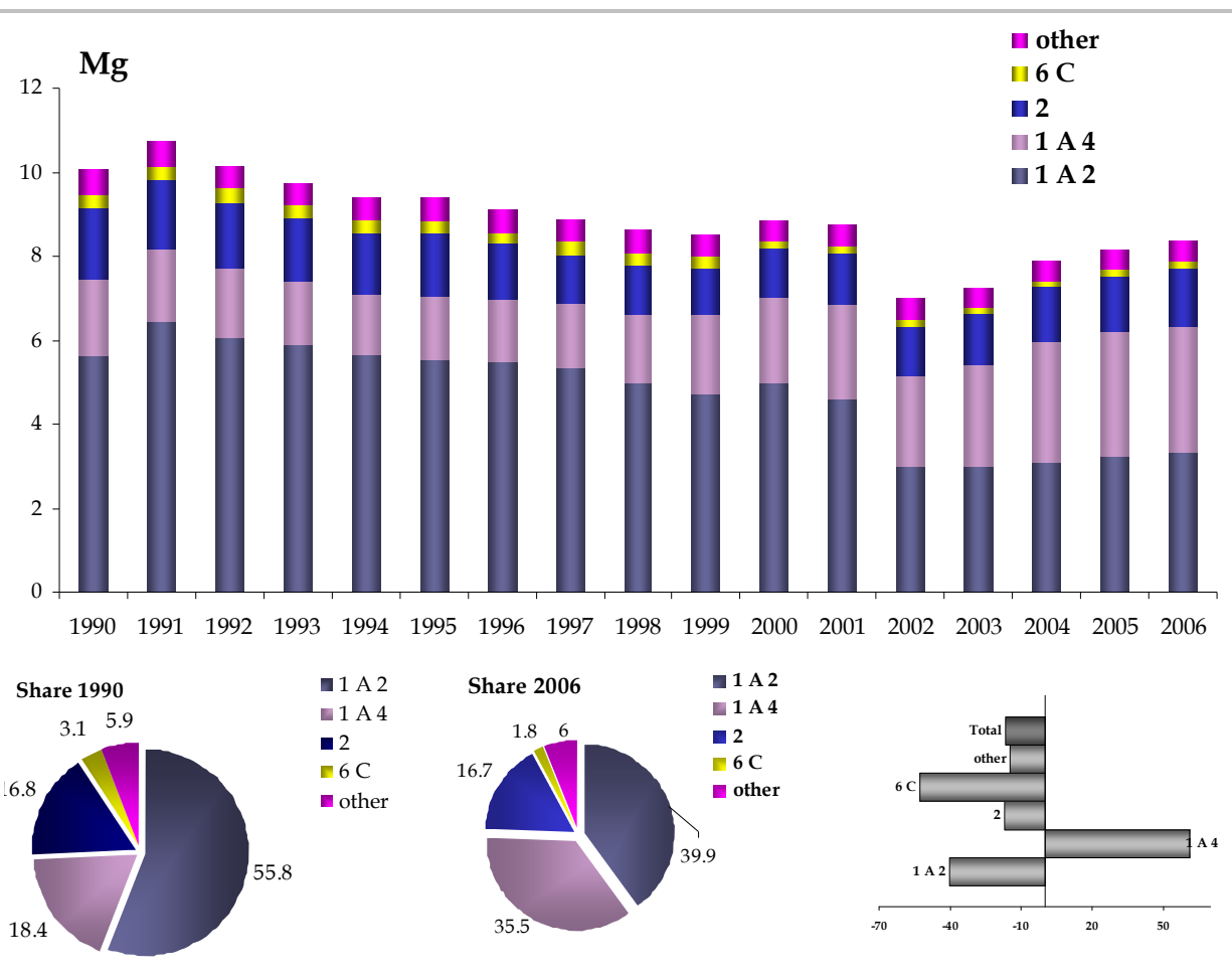
Figure 2.9 Cd emission trend 1990-2006, percentage share by sector and variation 1990-2006
