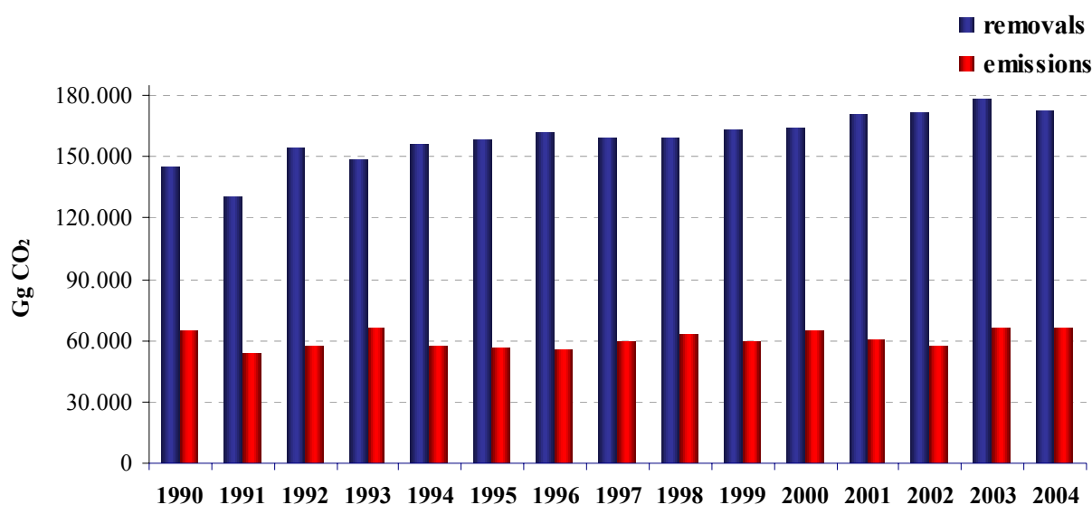
Figure 7.2 CO 2 removals and emissions in LULUCF sector in 2004 [Gg CO 2 ]
